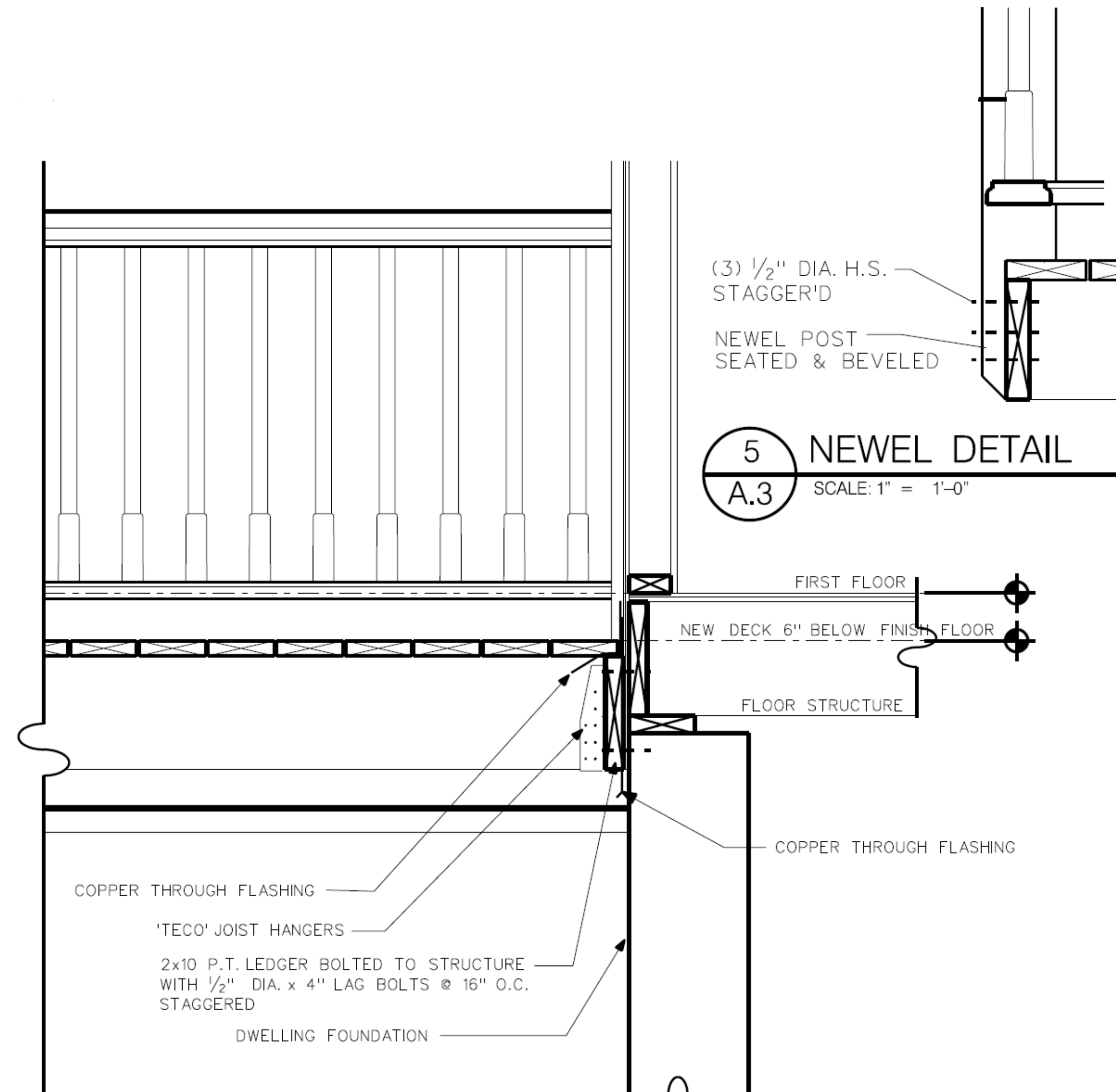
4 SECTION & DETAIL THRU DECK & DWELLING
