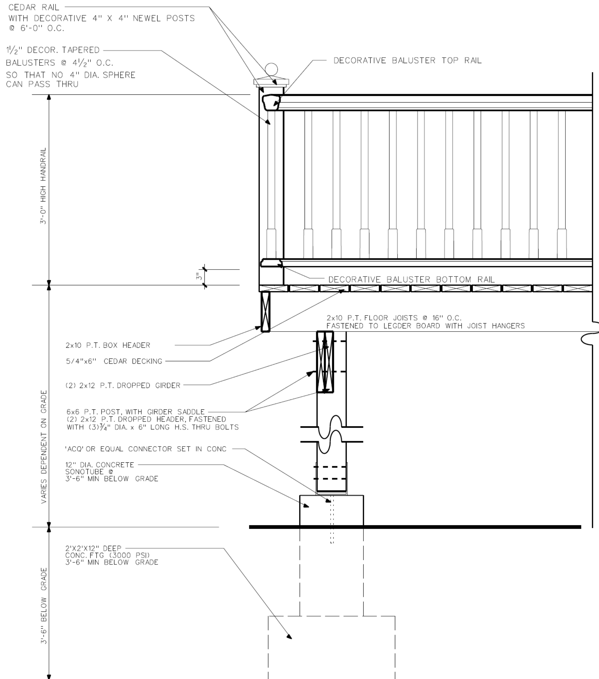
3 SECTION & DETAIL THRU DECK
