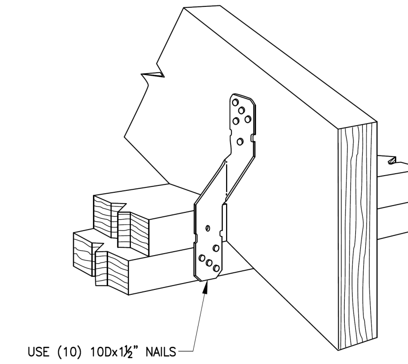
1 RAFTER TO TOP PLATES
